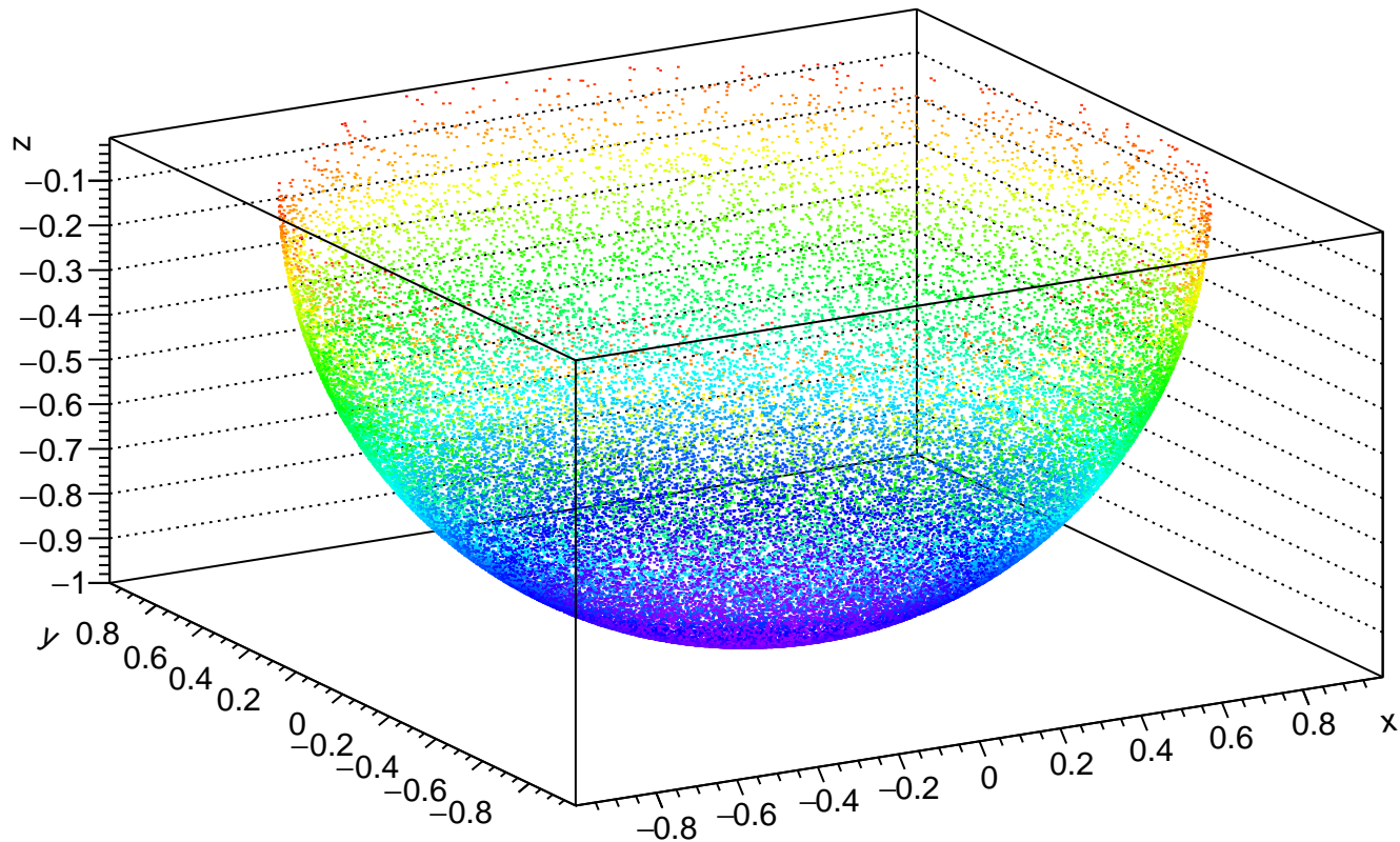
Plot of the 3-D distribution of rays exiting the port at the bottom of the sphere (false color)
