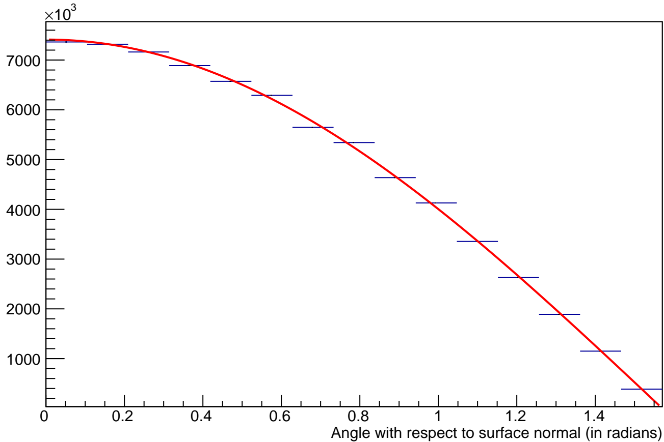
Distribution of angle w.r.t. surface normal of rays leaving the surface of the sphere
